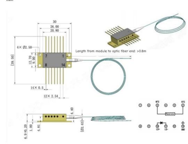
Outline drawings
